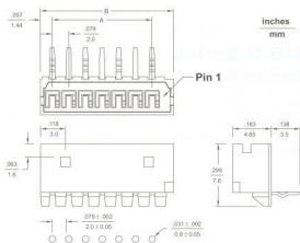
P. C. board hole dimensions
