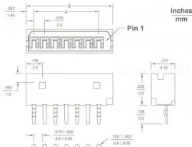
P. C. board hole dimensions
