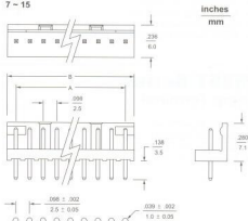
P. C. board hole dimensions
