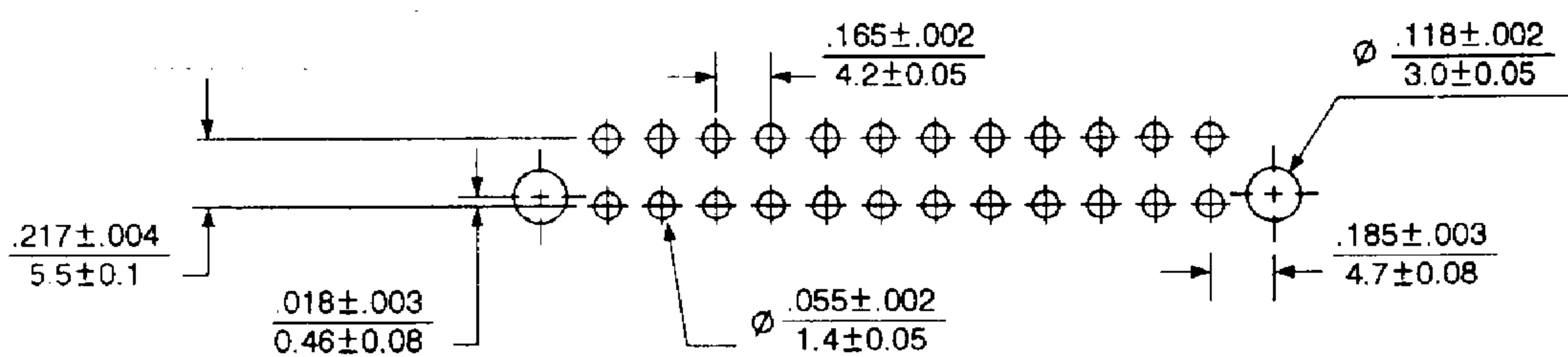
Vertical Header with Pegs P.C.B. Dimensions
