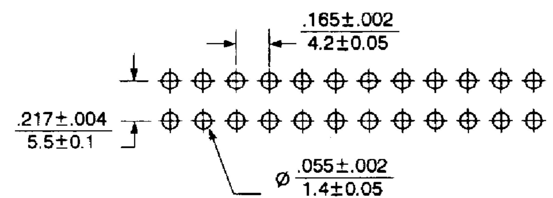
Vertical Header without Pegs P.C.B. Dimensions
